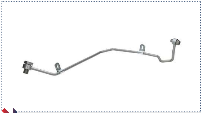
PT REF: PT-04-06-145 OEM REF: 7701476552 DESCRIPTION: OIL FEED PIPE BRAND: RENAULT MODEL: SCENIC / MEGANE / LAGUNA / GRAND / SCENIC YEAR: 2002-2024
