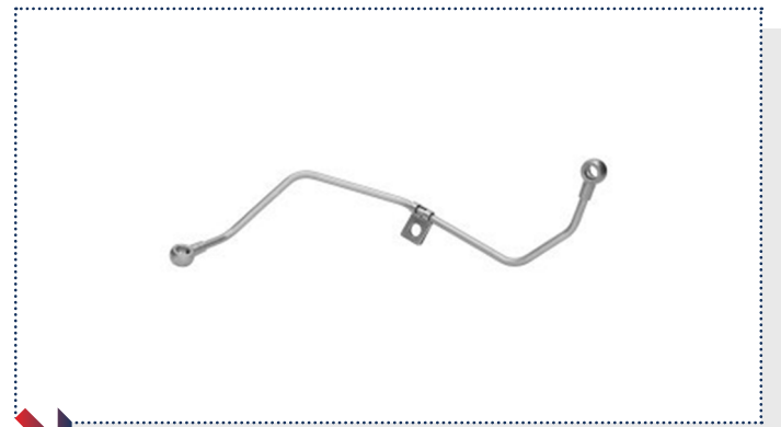
PT REF: PT-04-10-164 OEM REF: 282414A421 DESCRIPTION: OIL FEED PIPE BRAND: HYUNDAI / KIA MODEL: SORENTO JC / H1 TRAVEL / H1 STAREX / H-1 CARGO YEAR: 2002-2024
