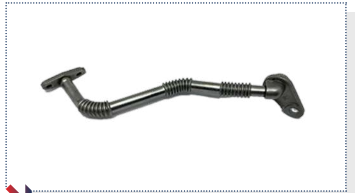
PT REF: PT-04-05-023 OEM REF: 55230879 - 55206325 DESCRIPTION: TURBO RETURN PIPE BRAND: FIAT MODEL: BRAVO2 / FREEMONT YEAR: 2008-2020
