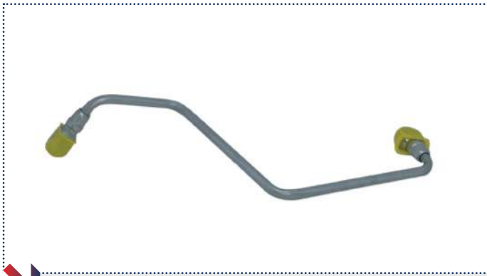
PT REF: PT-04-01-053 OEM REF: 2S6Q6K679AE - 1479851 - 0379.62 DESCRIPTION: OIL FEED PIPE BRAND: FORD / PSA MODEL: 206 / 207 / C3 / C1 / C2 / 307 / BIPPER / 1007 YEAR: 2001-2024
