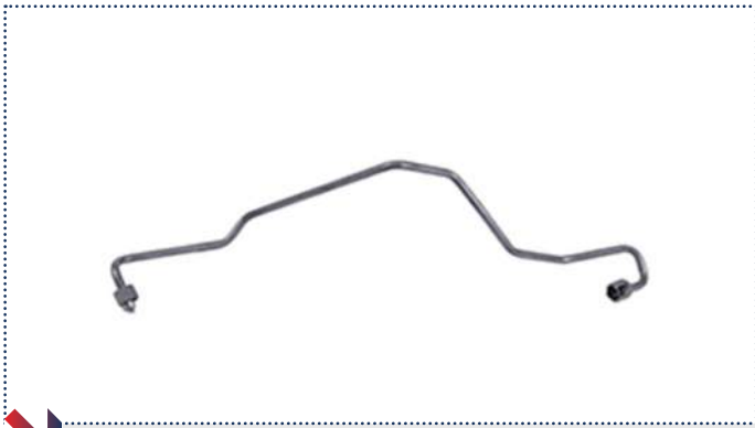
PT REF: PT-04-03-101 OEM REF: 03G145771J DESCRIPTION: OIL FEED PIPE BRAND: VW MODEL: GOLF / POLO / A3 / TOURAN / PASSAT / IBZA / A3 / CADDY / FABIA / ALTEA YEAR: 2001-2024
