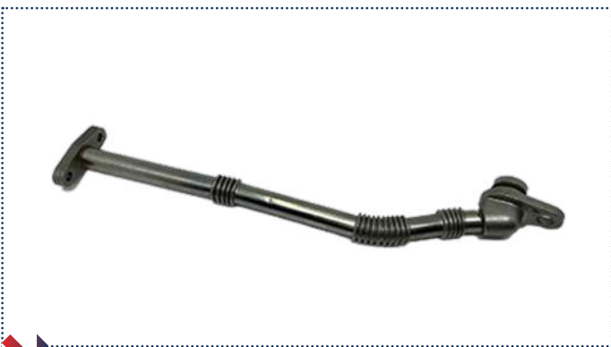
PT REF: PT-04-09-063 OEM REF: 55500870 DESCRIPTION: TURBO RETURN PIPE BRAND: OPEL MODEL: ASTRA / MOKKA / MERIVA / NSIGNIA YEAR: 2013-2024
